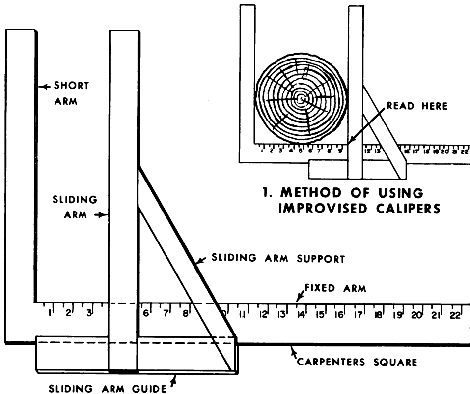
Figure 2-7. Improvised calipers.
